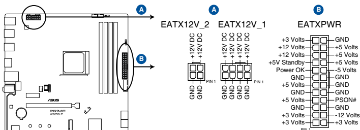
PRIME X570-P ATX power connectors
